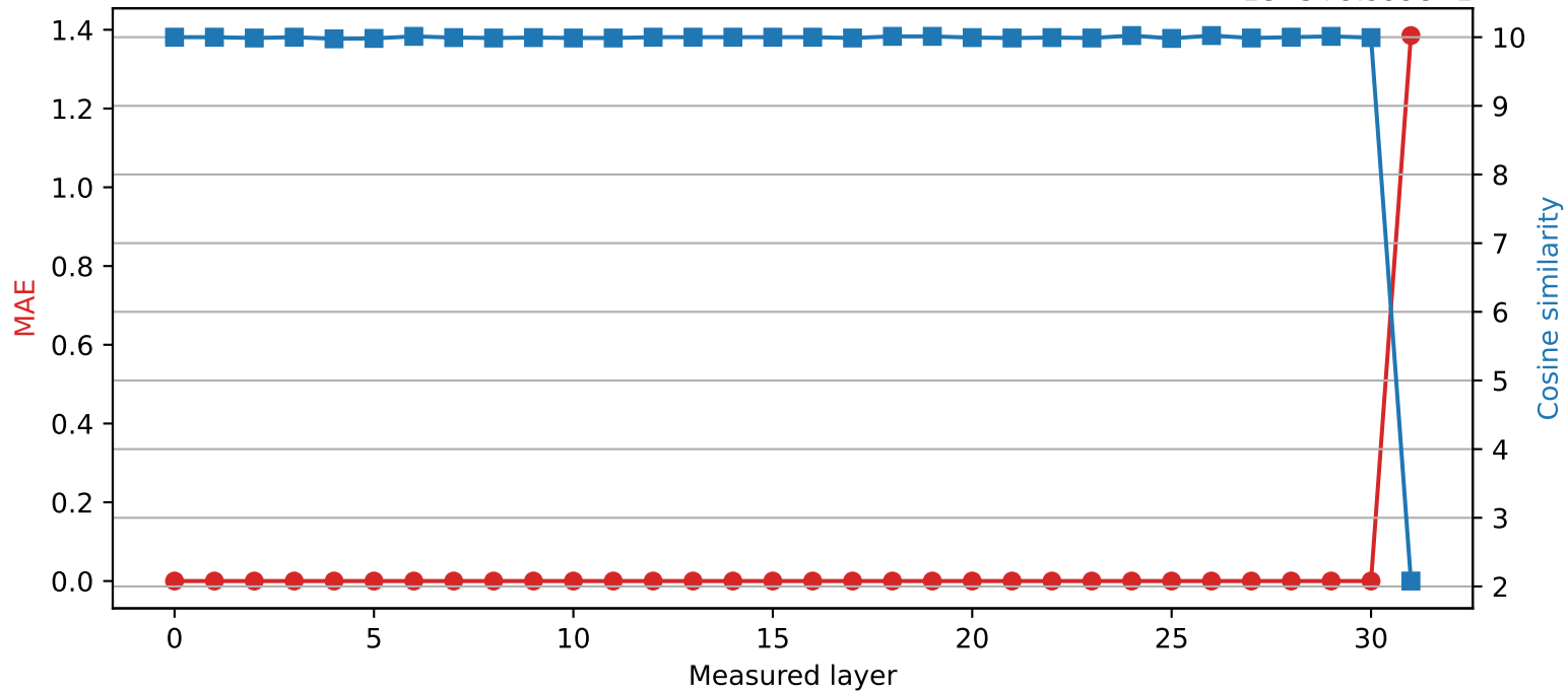
SmolLM2-360M | Quantized layer 30 | float32 \rightarrow int8 1e-5+9.999e-1
