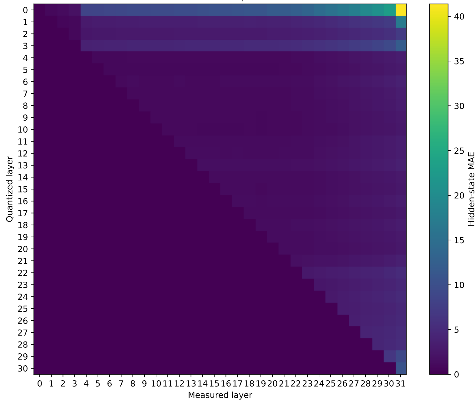
Model: SmolLM2-360M | float32 → int4
