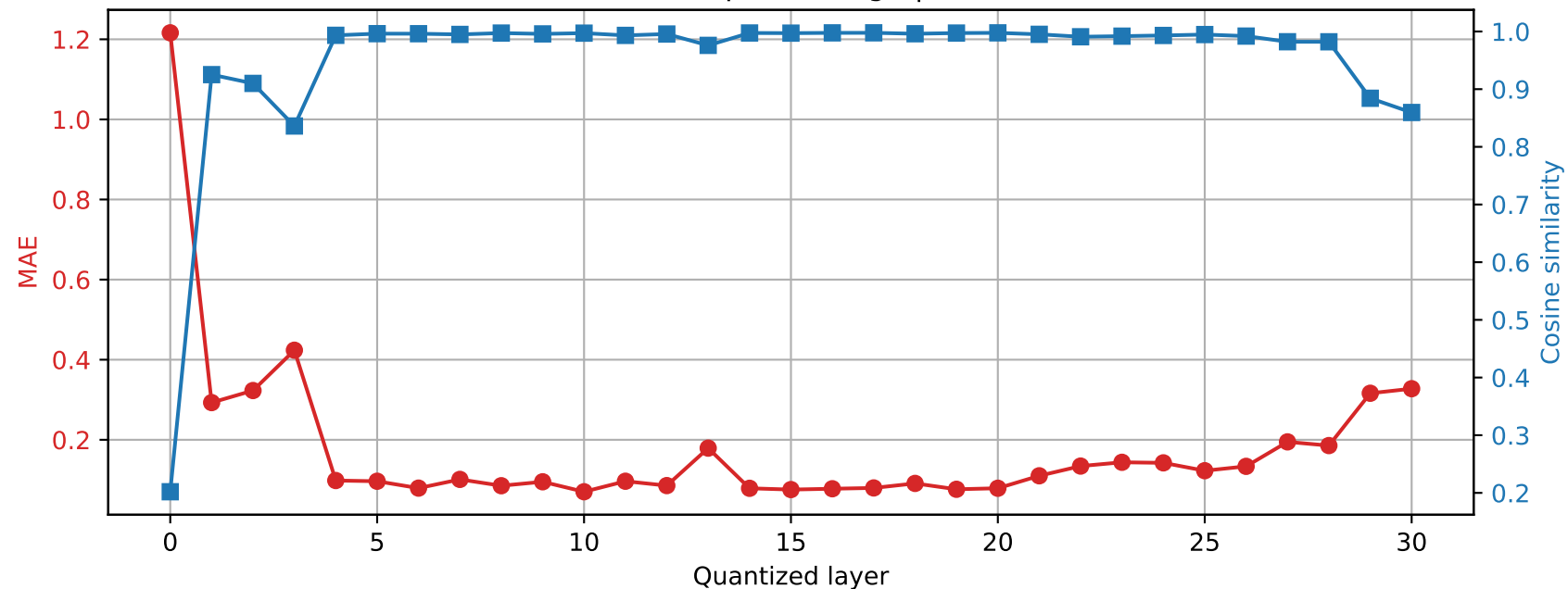
SmolLM2-360M | Prompt 0 Final RMSNorm output damage | float32 \rightarrow int4
