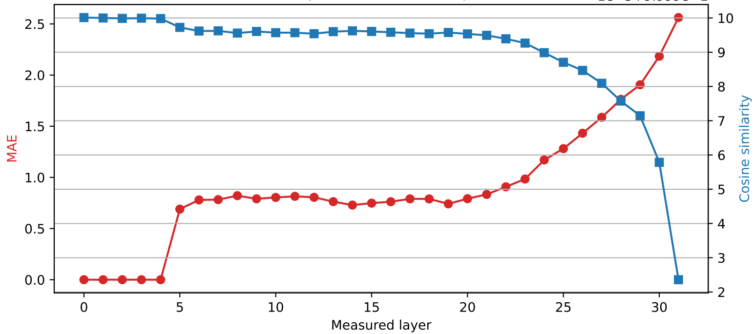
SmolLM2-360M | Quantized layer 4 | float32 → int4
