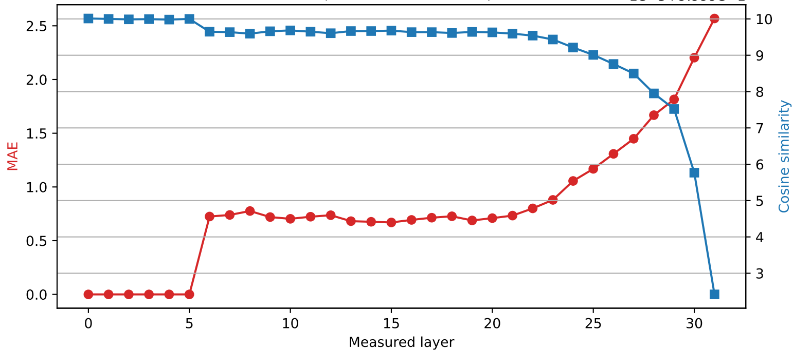
SmolLM2-360M | Quantized layer 5 | float32 → int4
