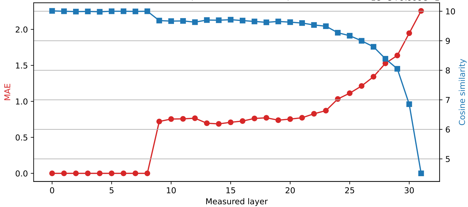
SmolLM2-360M | Quantized layer 8 | float32 → int4
