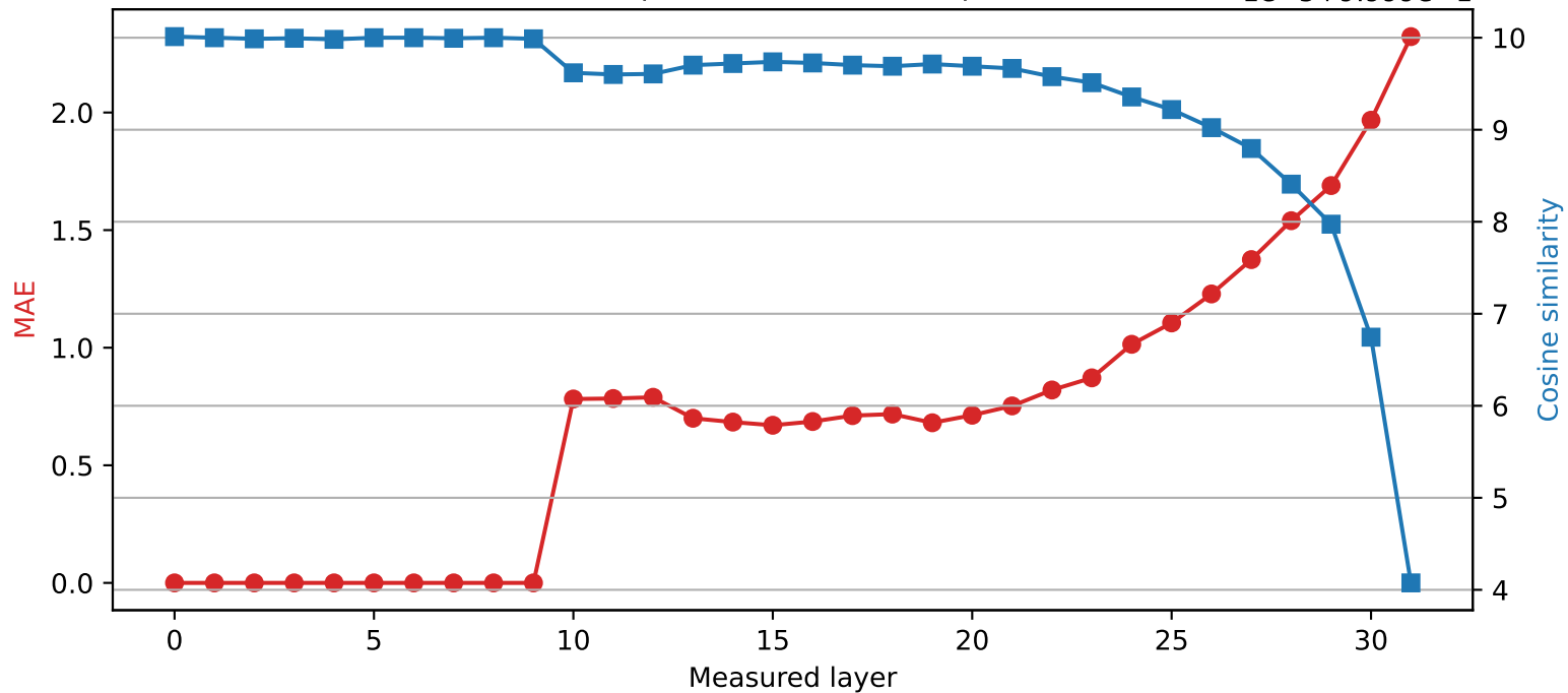
SmolLM2-360M | Quantized layer 9 | float32 → int4
