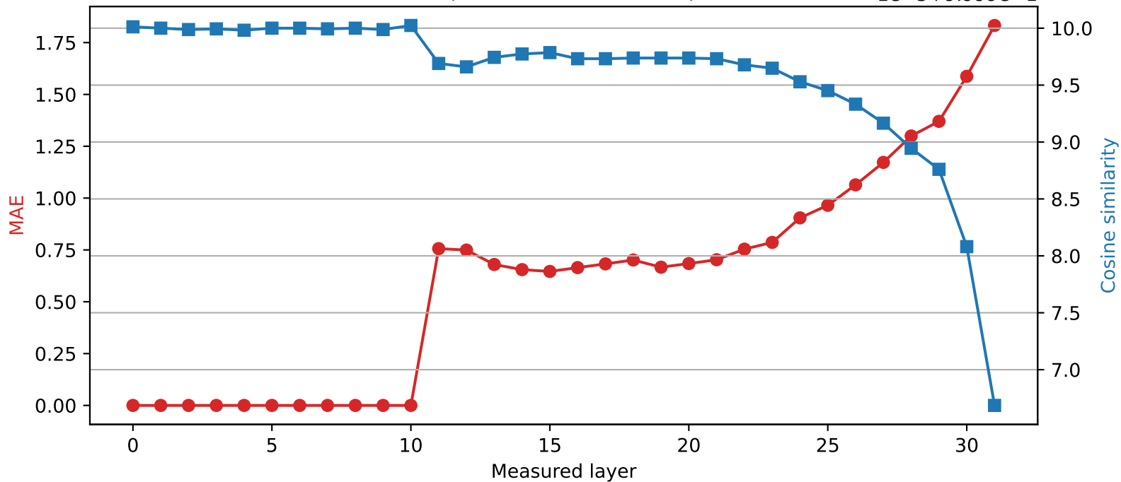
SmolLM2-360M | Quantized layer 10 | float32 → int4 1e-5+9.999e-1
