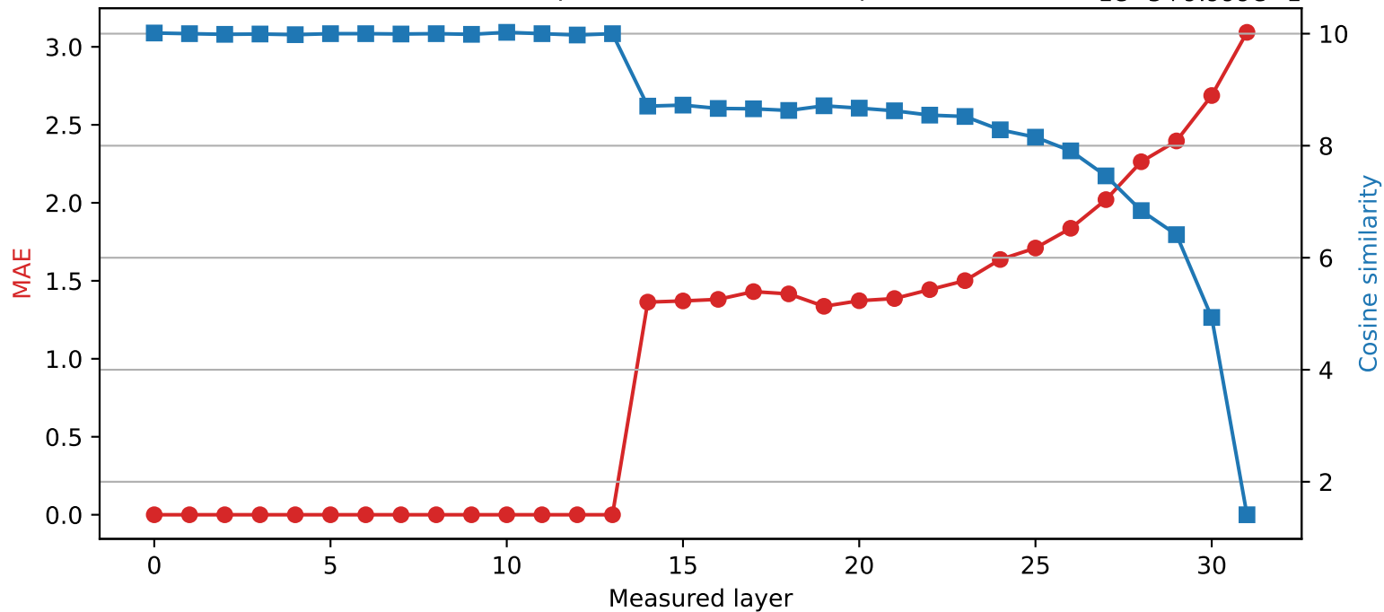
SmolLM2-360M | Quantized layer 13 | float32 \rightarrow int4 1e-5+9.999e-1
