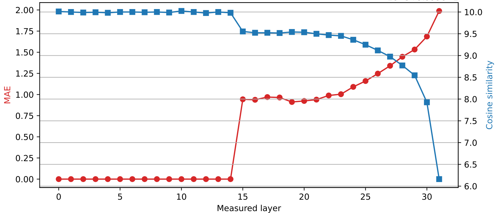
SmolLM2-360M | Quantized layer 14 | float32 \rightarrow int4 1e-5+9.999e-1
