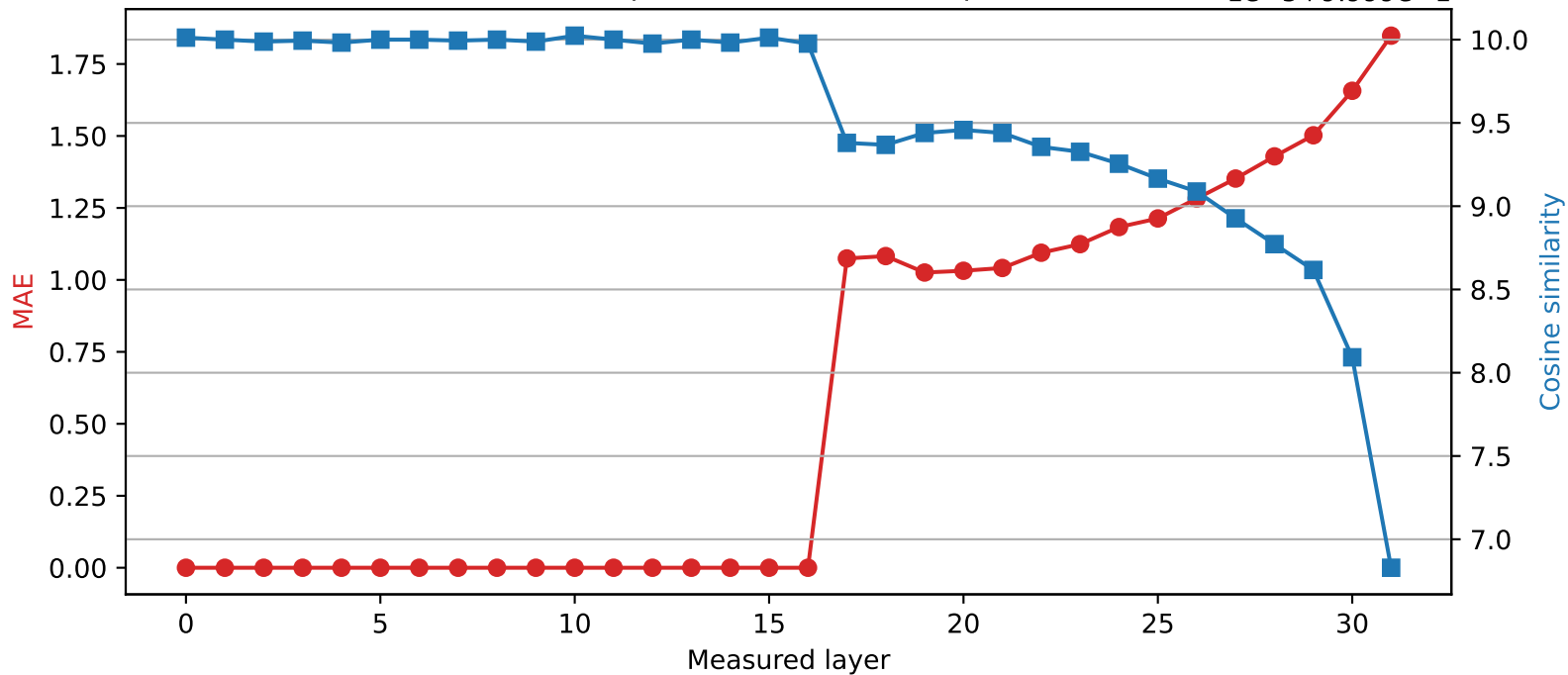
SmolLM2-360M | Quantized layer 16 | float32 \rightarrow int4 1e-5+9.999e-1
