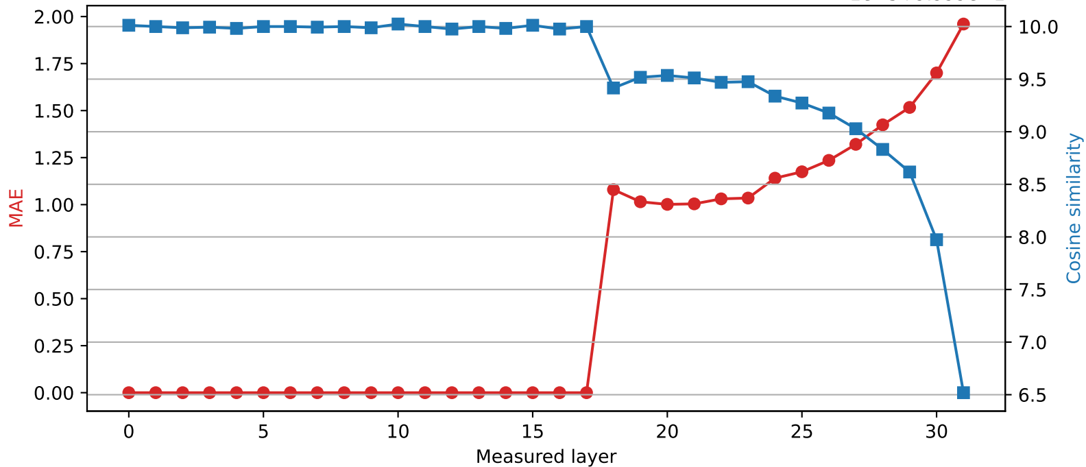
SmolLM2-360M | Quantized layer 17 | float32 \rightarrow int4 1e-5+9.999e-1
