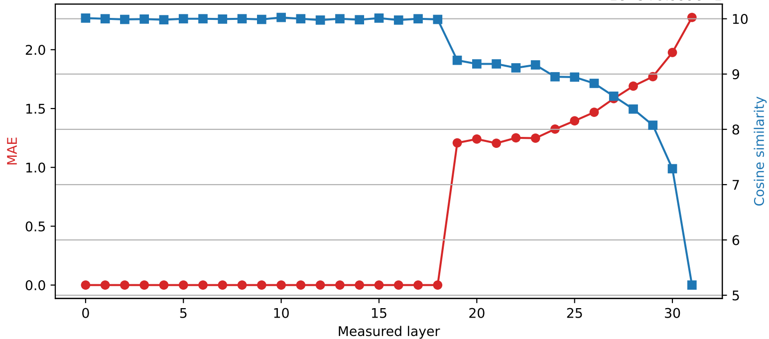
SmolLM2-360M | Quantized layer 18 | float32 \rightarrow int4 1e-5+9.999e-1
