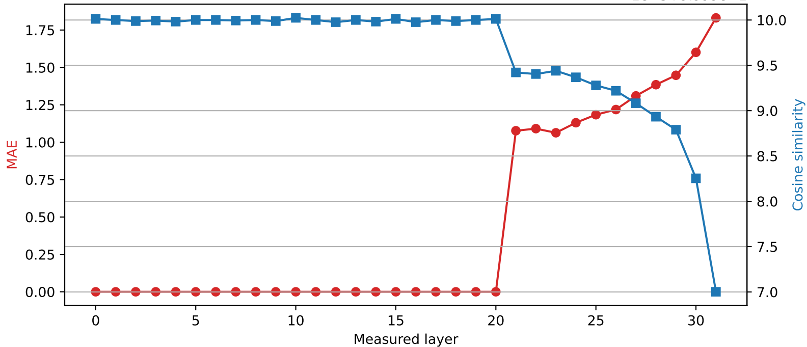
SmolLM2-360M | Quantized layer 20 | float32 \rightarrow int4 1e-5+9.999e-1
