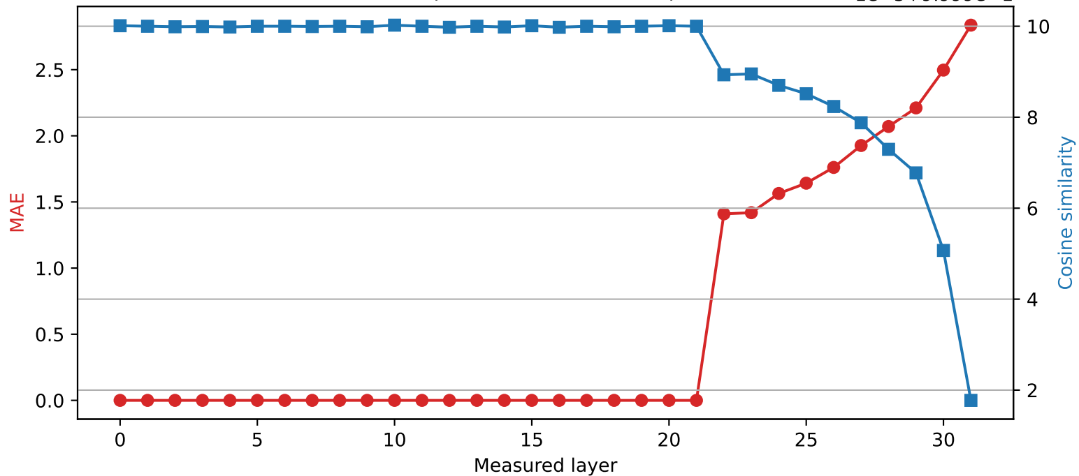
SmolLM2-360M | Quantized layer 21 | float32 \rightarrow int4 1e-5+9.999e-1
