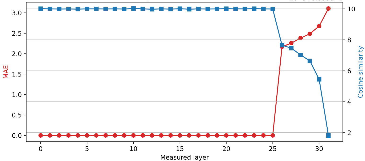
SmolLM2-360M | Quantized layer 25 | float32 \rightarrow int4 1e-5+9.999e-1
