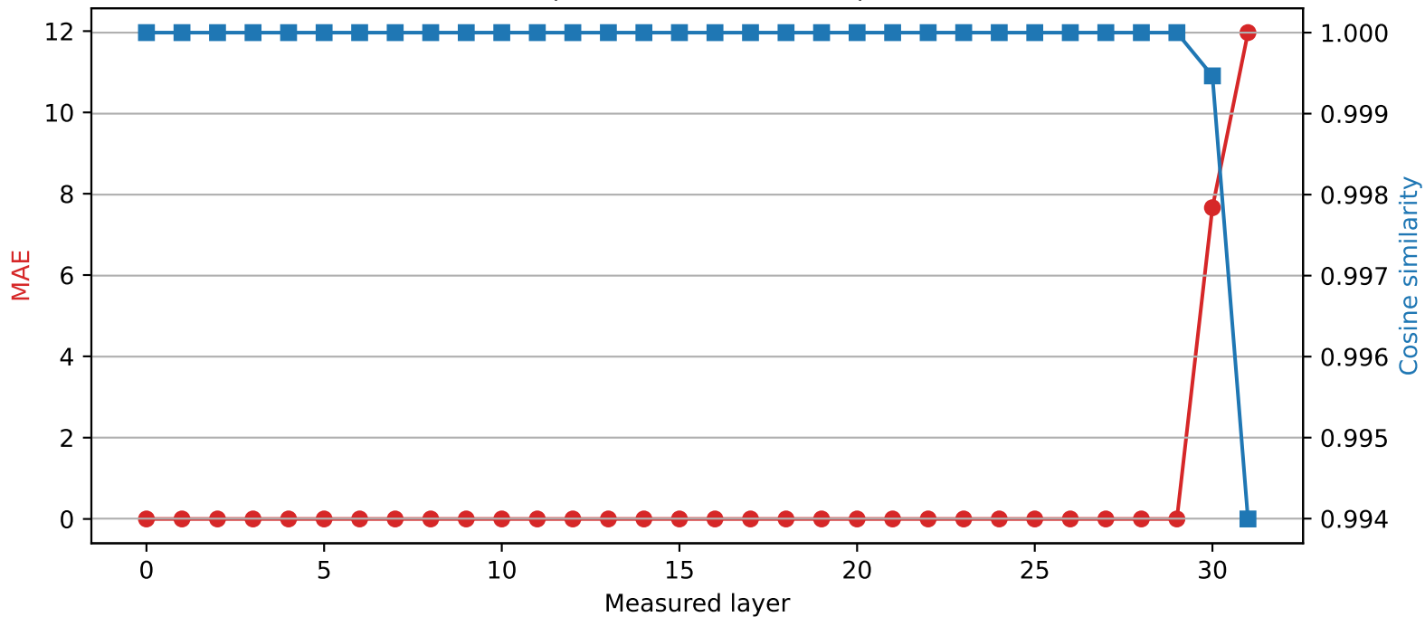
SmolLM2-360M | Quantized layer 29 | float32 \rightarrow int4
