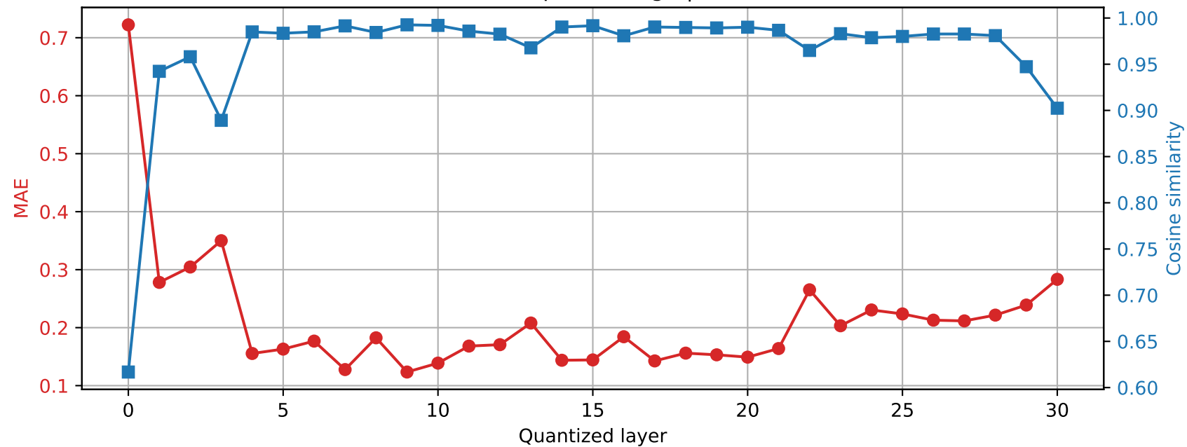
SmolLM2-360M | Prompt 1 Final RMSNorm output damage | float32 → int4
