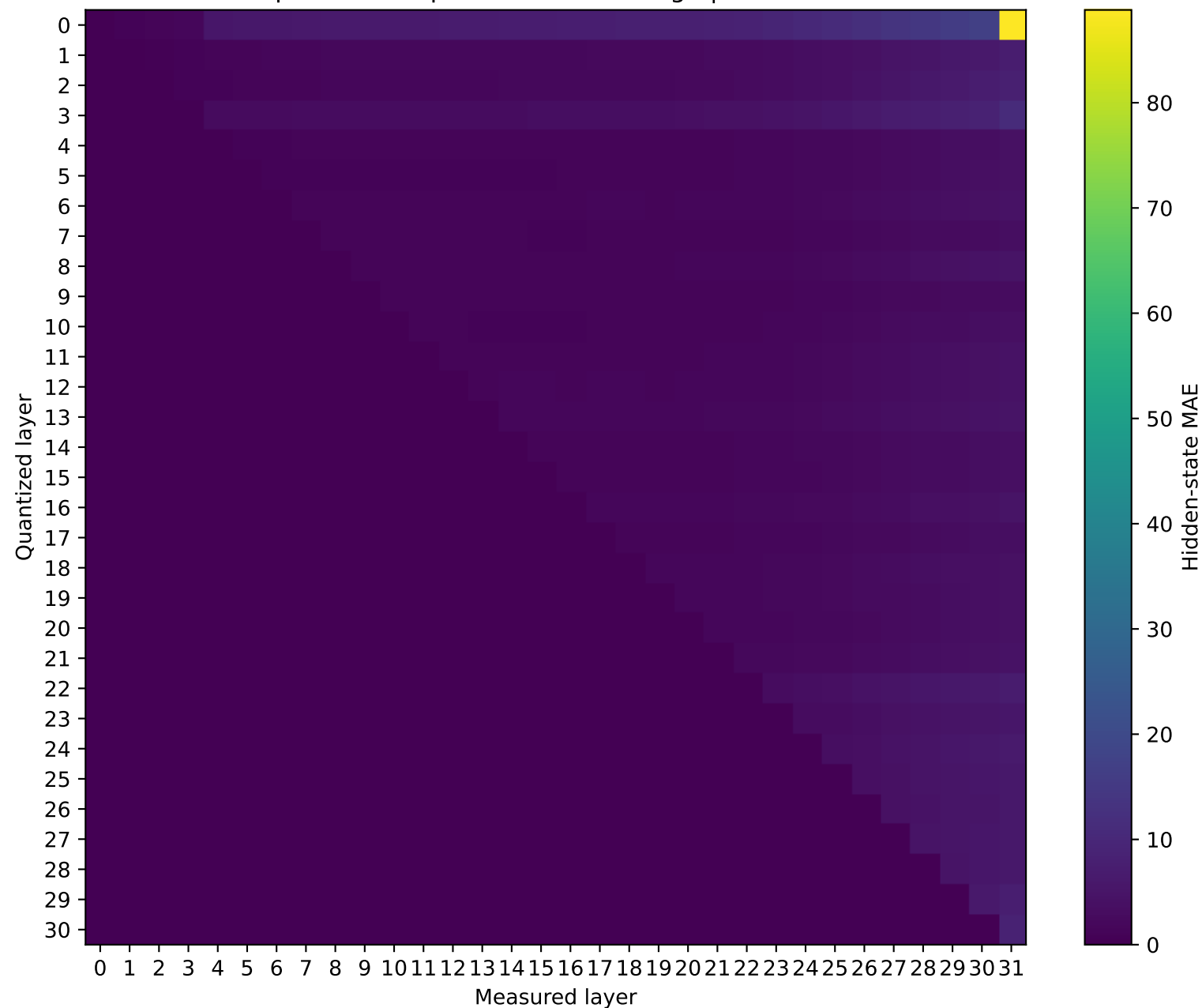
SmolLM2-360M
