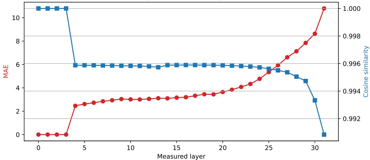
SmolLM2-360M | Quantized layer 3 | float32 → int4
