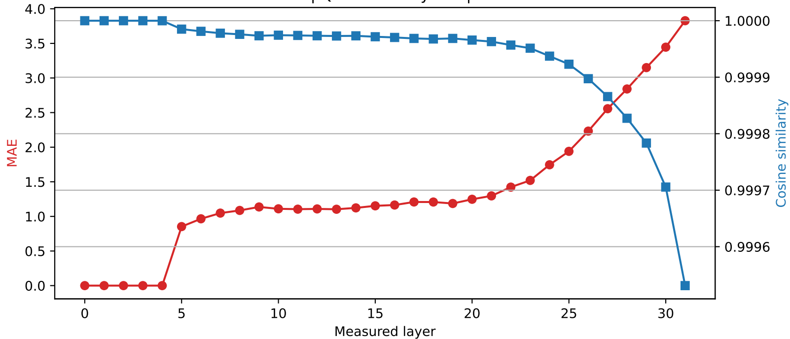
SmolLM2-360M | Quantized layer 4 | float32 \rightarrow int4
