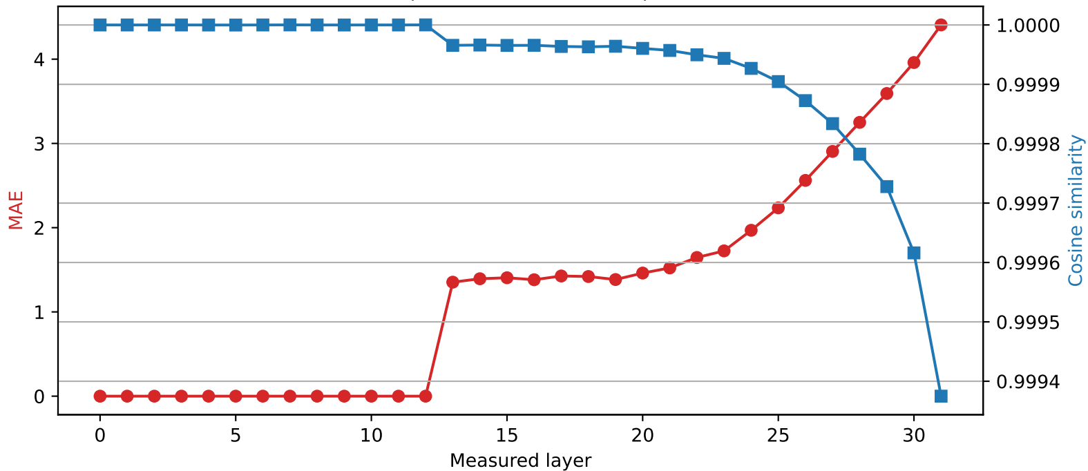
SmolLM2-360M | Quantized layer 12 | float32 → int4
