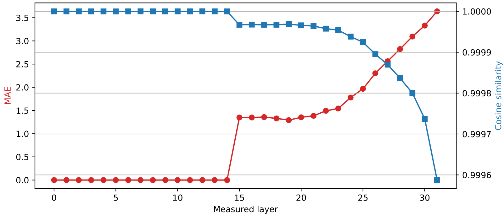
SmolLM2-360M | Quantized layer 14 | float32 \rightarrow int4
