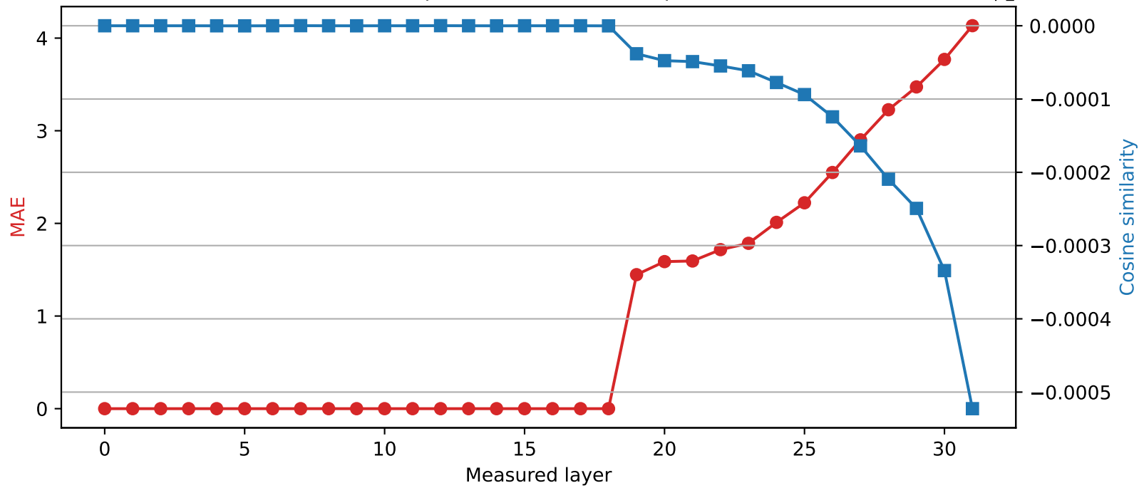
SmolLM2-360M | Quantized layer 18 | float32 \rightarrow int4
