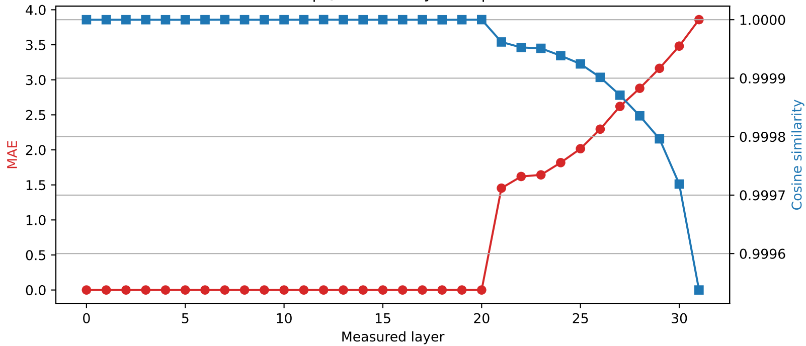
SmolLM2-360M | Quantized layer 20 | float32 \rightarrow int4
