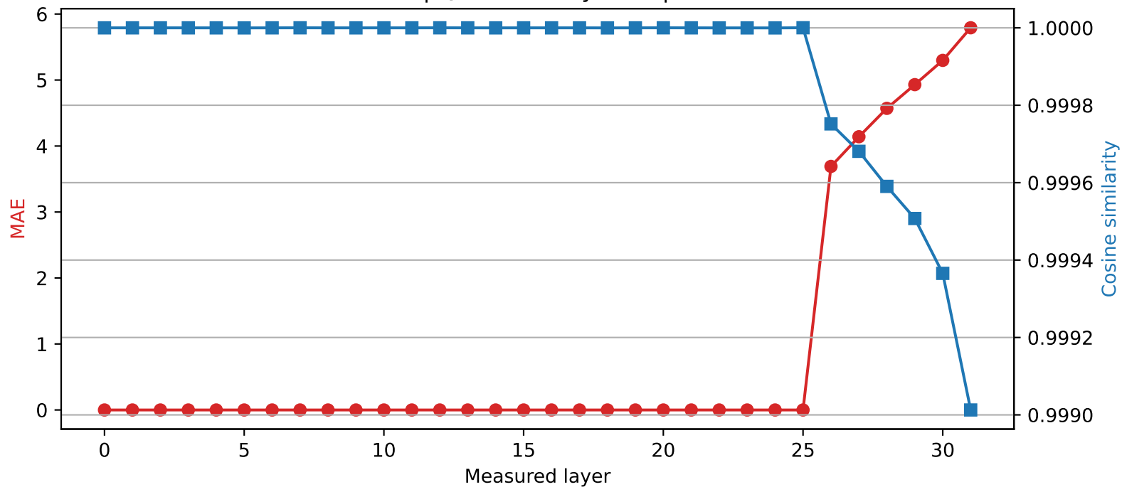
SmolLM2-360M | Quantized layer 25 | float32 \rightarrow int4
