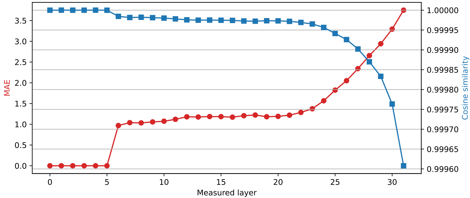
SmolLM2-360M | Quantized layer 5 | float32 \rightarrow int4
