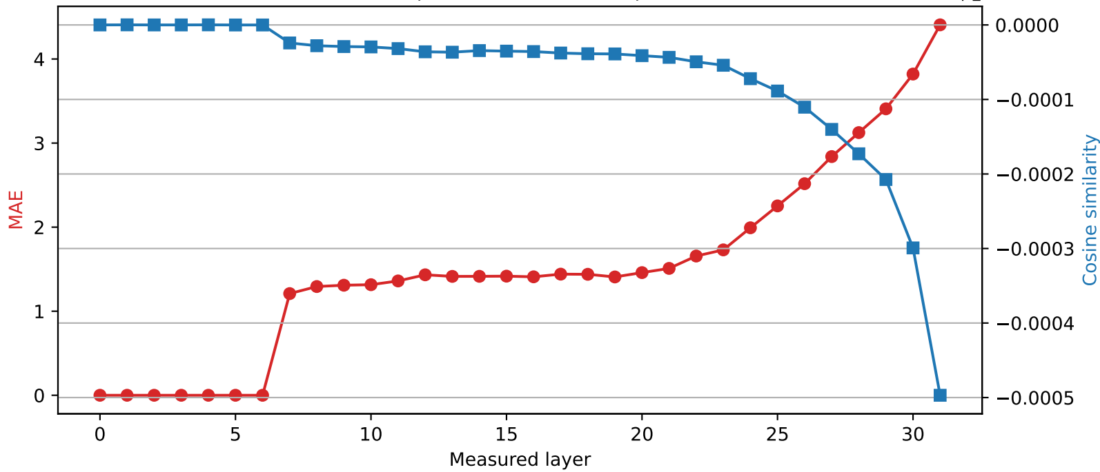
SmolLM2-360M | Quantized layer 6 | float32 \rightarrow int4
