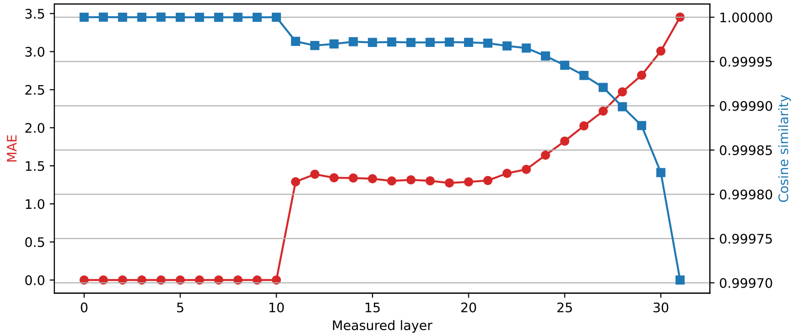
SmolLM2-360M | Quantized layer 10 | float32 \rightarrow int4
