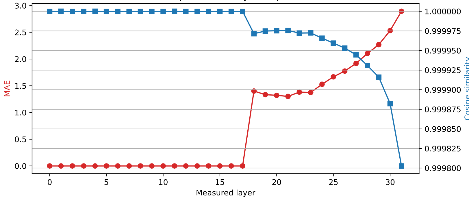
SmolLM2-360M | Quantized layer 17 | float32 → int4
