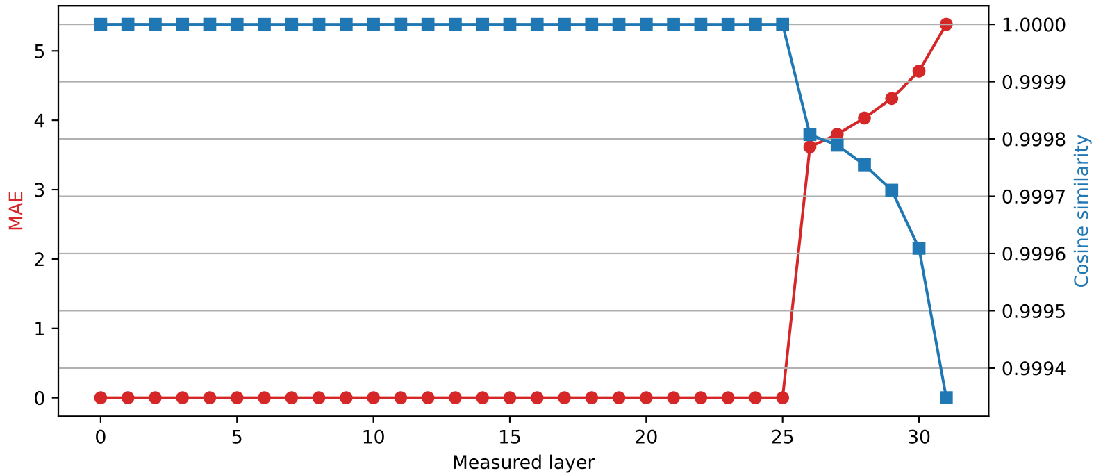
SmolLM2-360M | Quantized layer 25 | float32 → int4
