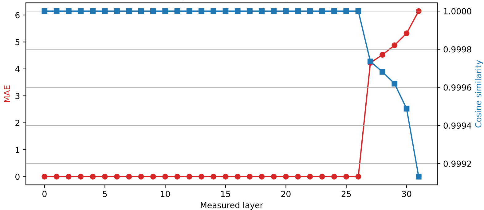
SmolLM2-360M | Quantized layer 26 | float32 \rightarrow int4
