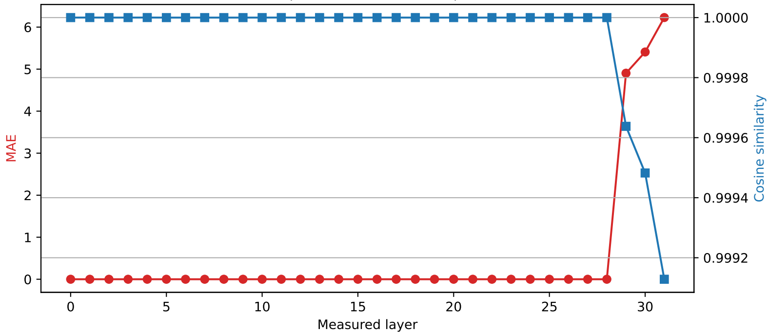
SmolLM2-360M | Quantized layer 28 | float32 \rightarrow int4
