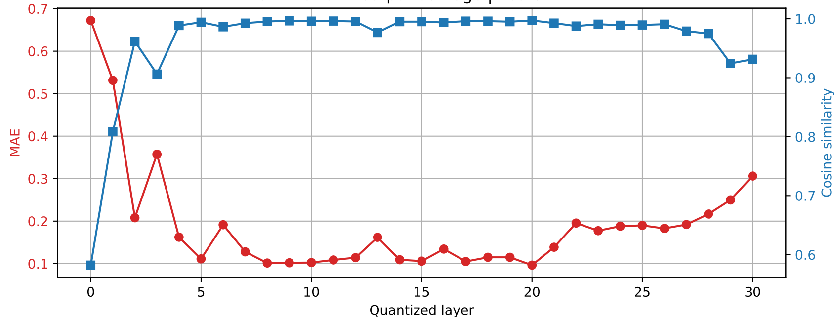
SmolLM2-360M | Prompt 3 Final RMSNorm output damage | float32 → int4
