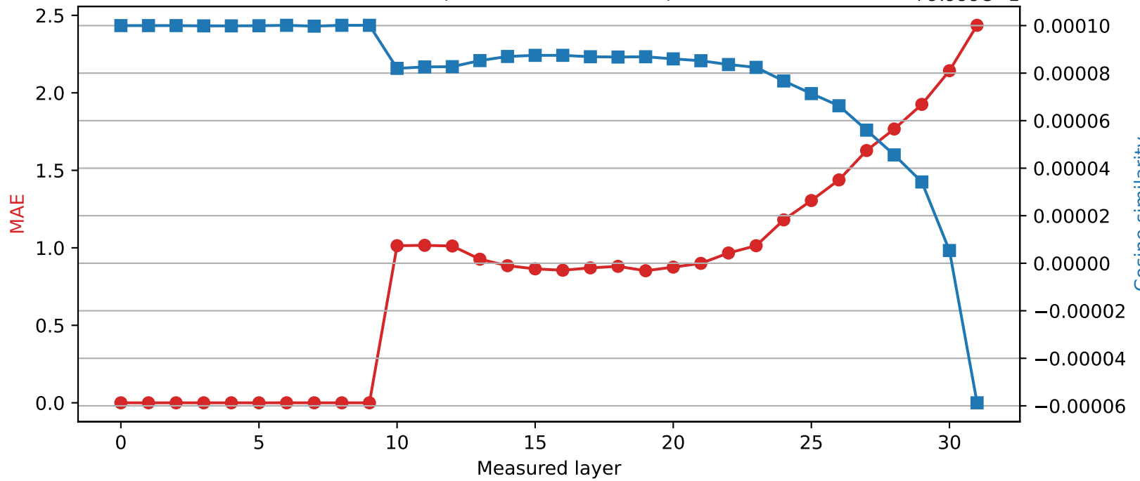
SmolLM2-360M | Quantized layer 9 | float32 \rightarrow int4
