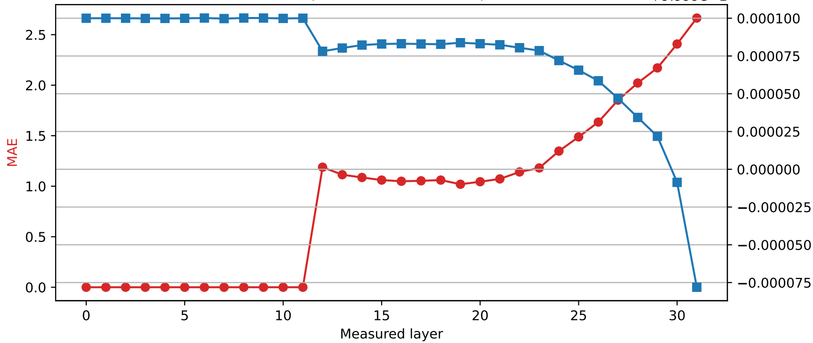
SmolLM2-360M | Quantized layer 11 | float32 → int4
