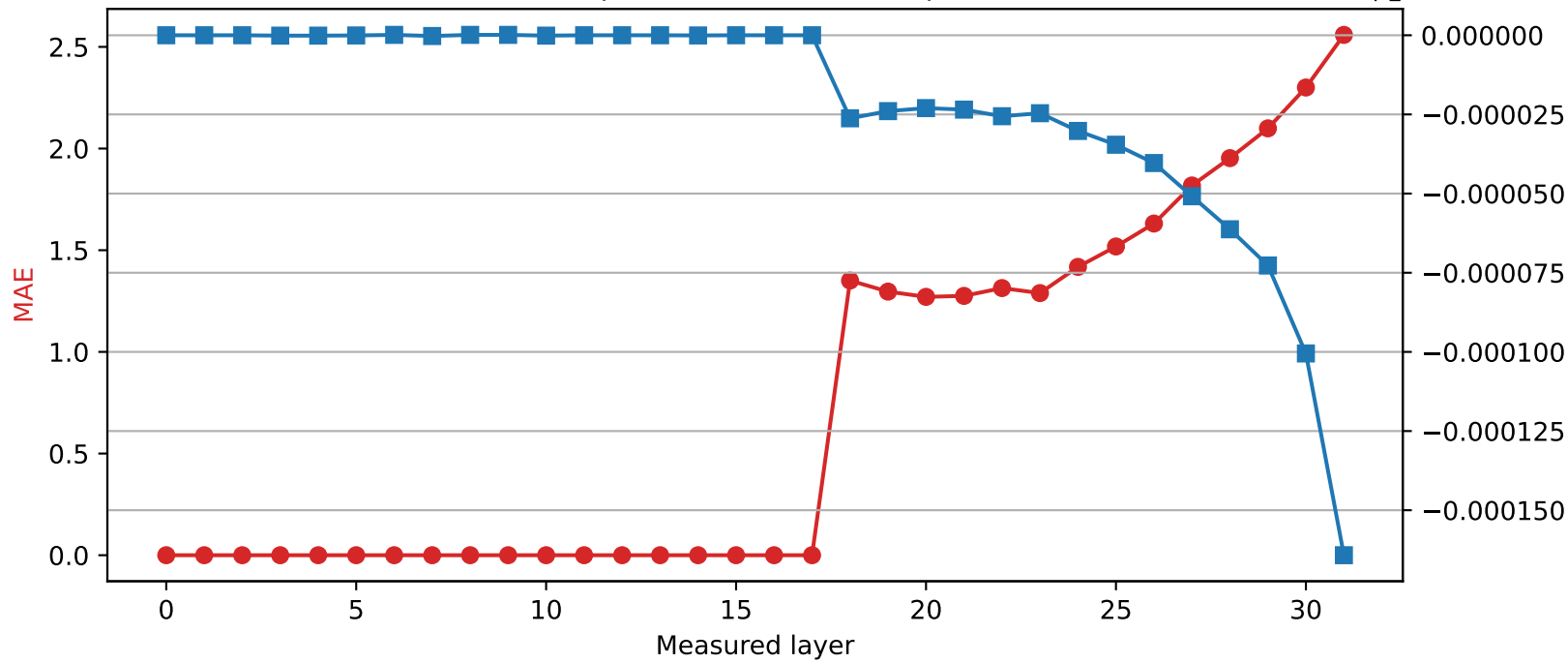
SmolLM2-360M | Quantized layer 17 | float32 \rightarrow int4
