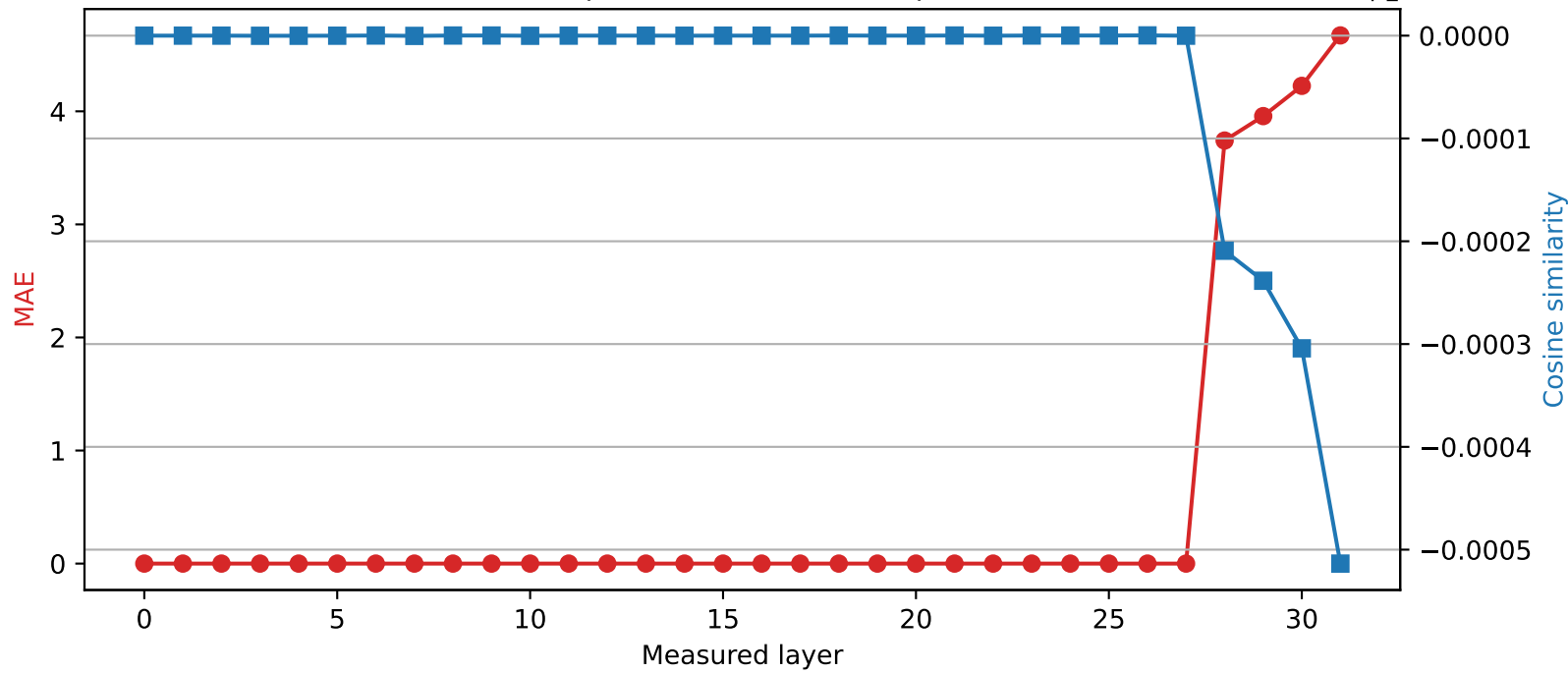
SmolLM2-360M | Quantized layer 27 | float32 → int4
