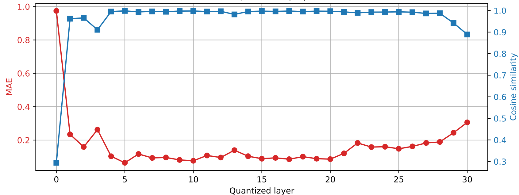
SmolLM2-360M | Prompt 4 Final RMSNorm output damage | float32 → int4
