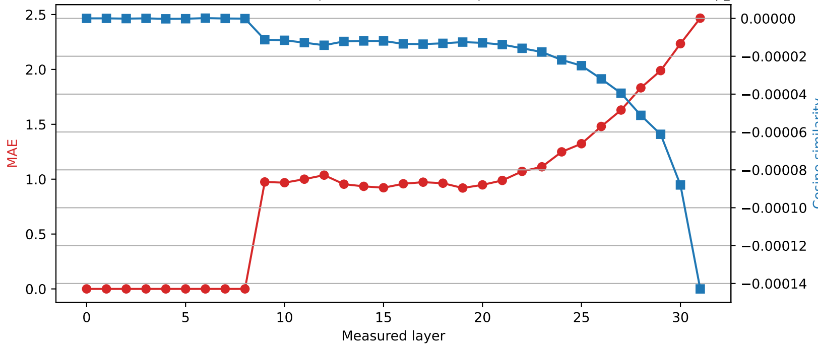
SmolLM2-360M | Quantized layer 8 | float32 \rightarrow int4
