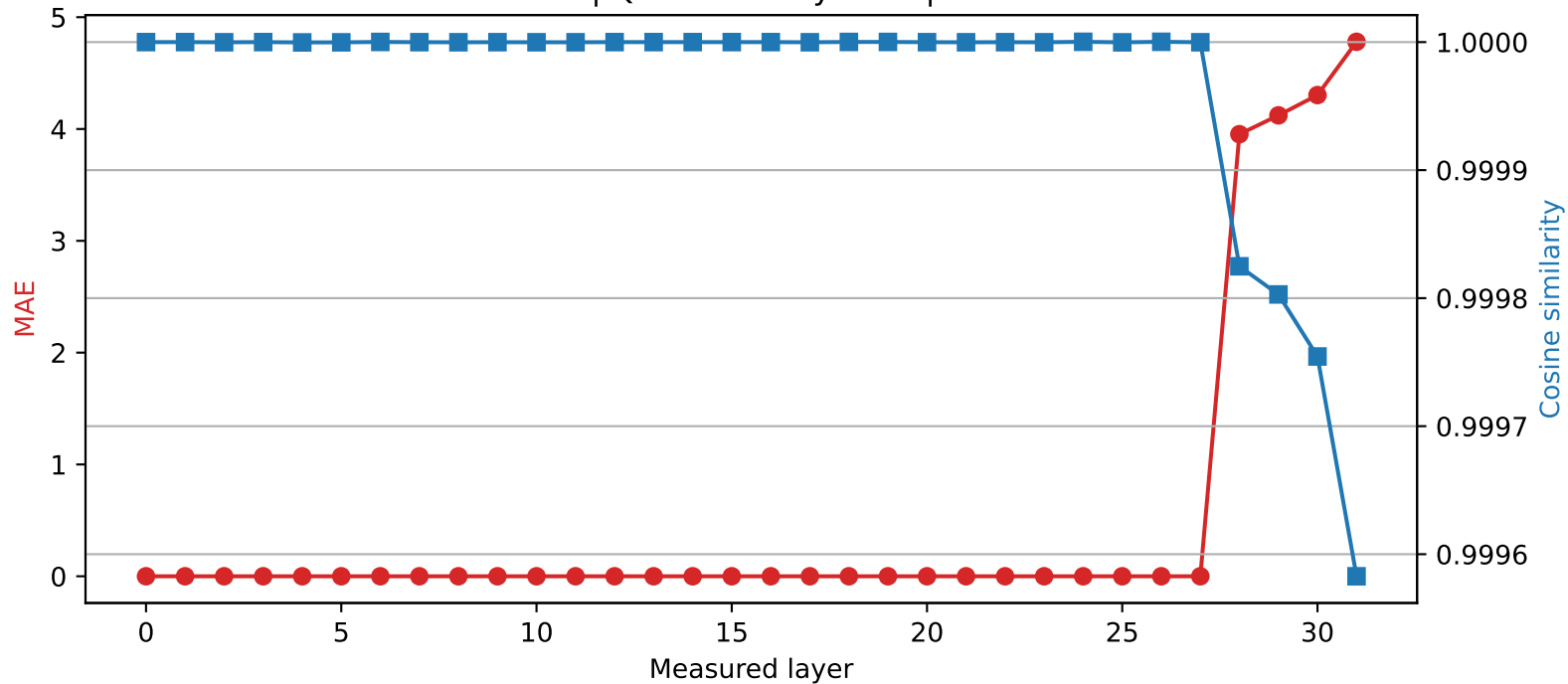
SmolLM2-360M | Quantized layer 27 | float32 \rightarrow int4
