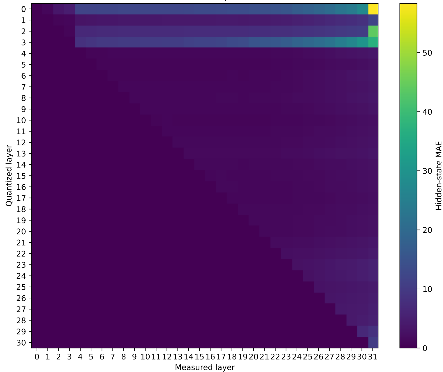
Model: SmolLM2-360M | float32 → int2
