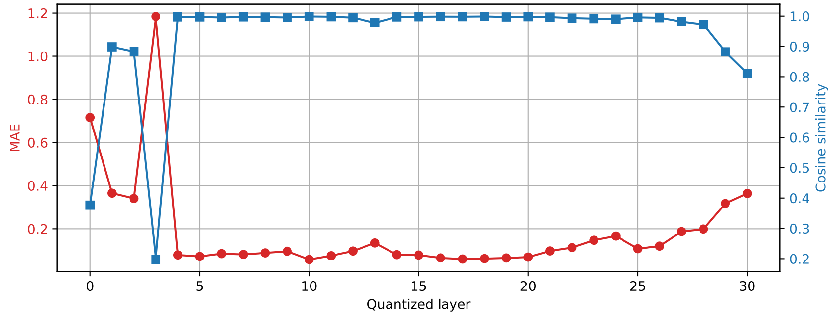
SmolLM2-360M | Prompt 0 Final RMSNorm output damage | float32 → int2
