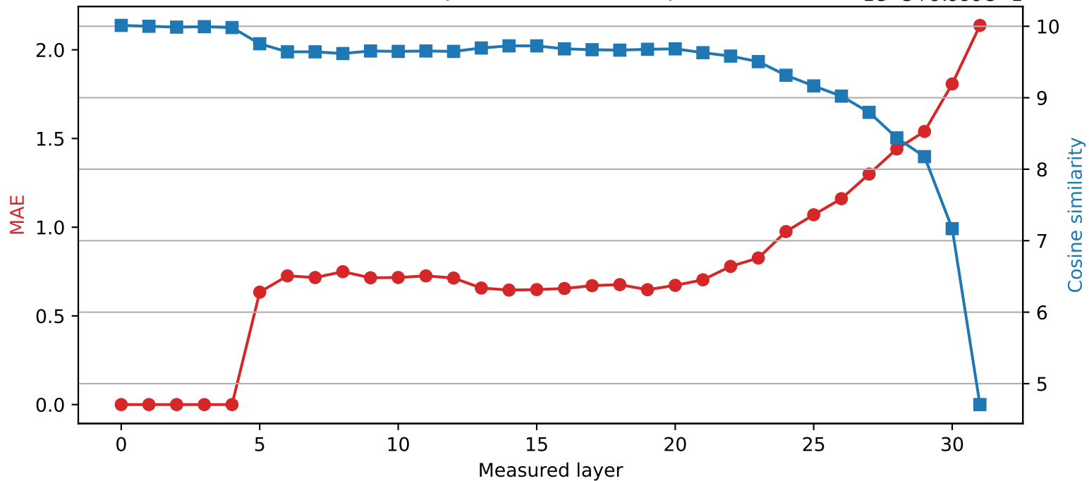
SmolLM2-360M | Quantized layer 4 | float32 → int2
