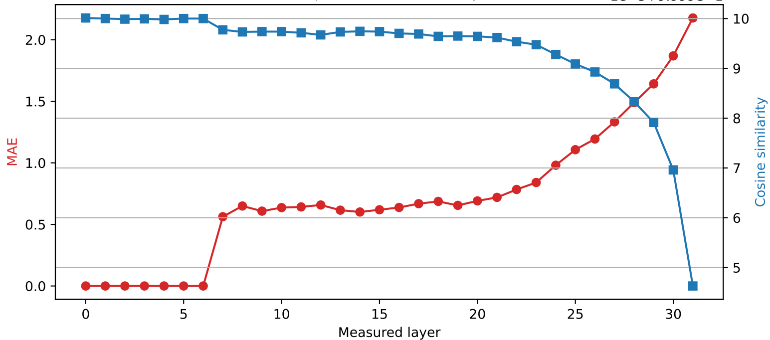
SmolLM2-360M | Quantized layer 6 | float32 → int2
