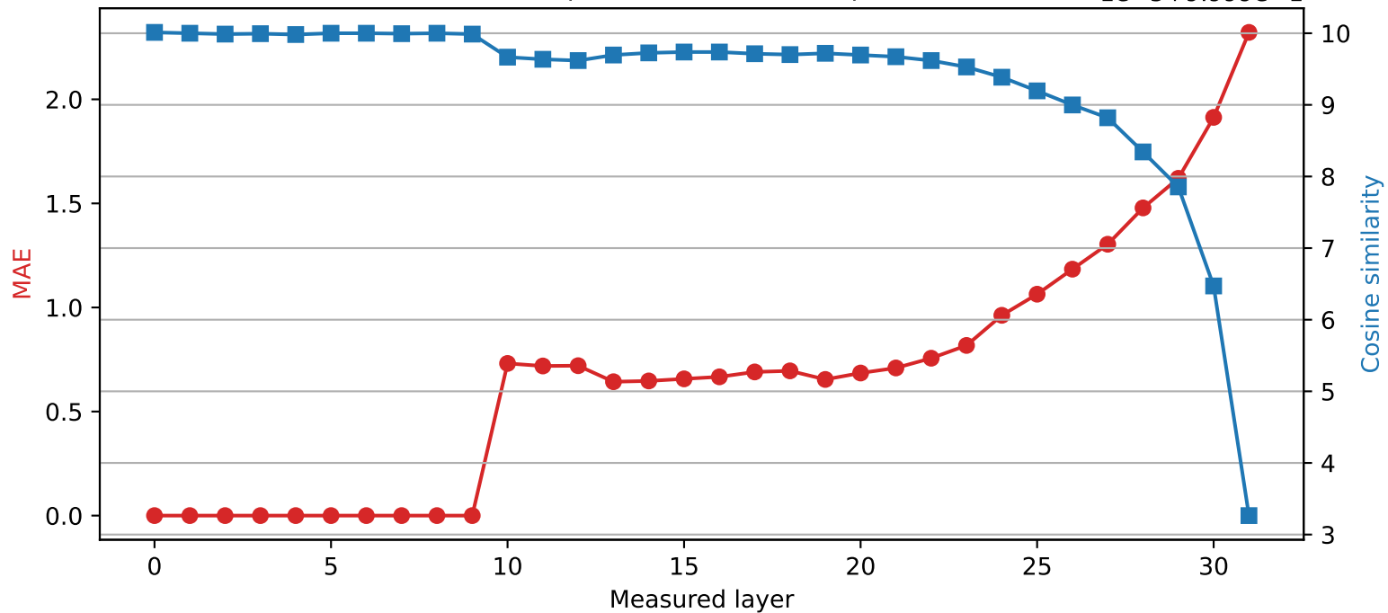
SmolLM2-360M | Quantized layer 9 | float32 → int2
