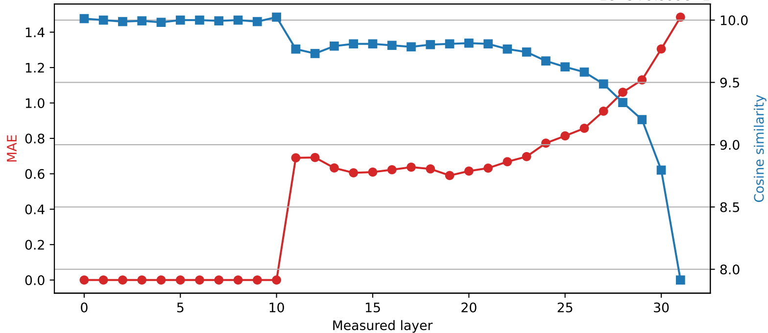
SmolLM2-360M | Quantized layer 10 | float32 \rightarrow int2 1e-5+9.999e-1
