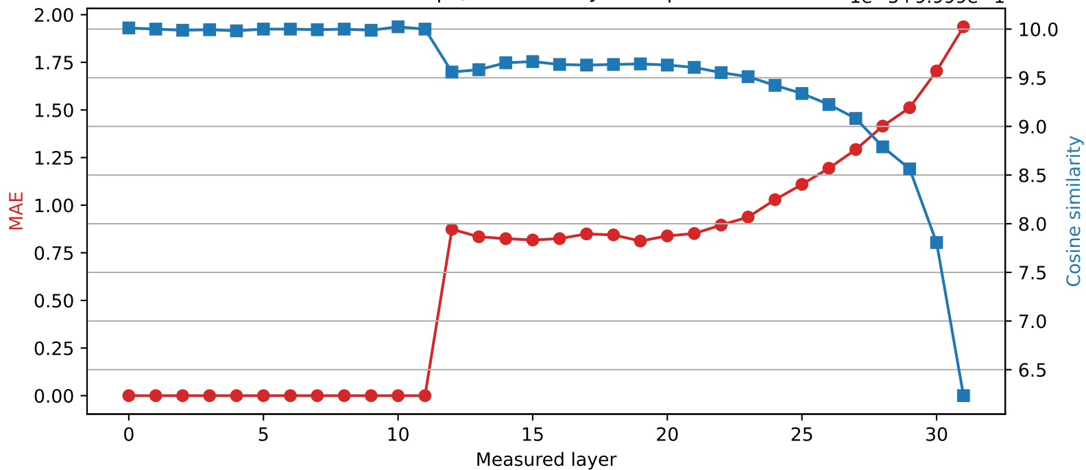
SmolLM2-360M | Quantized layer 11 | float32 \rightarrow int2 1e-5+9.999e-1
