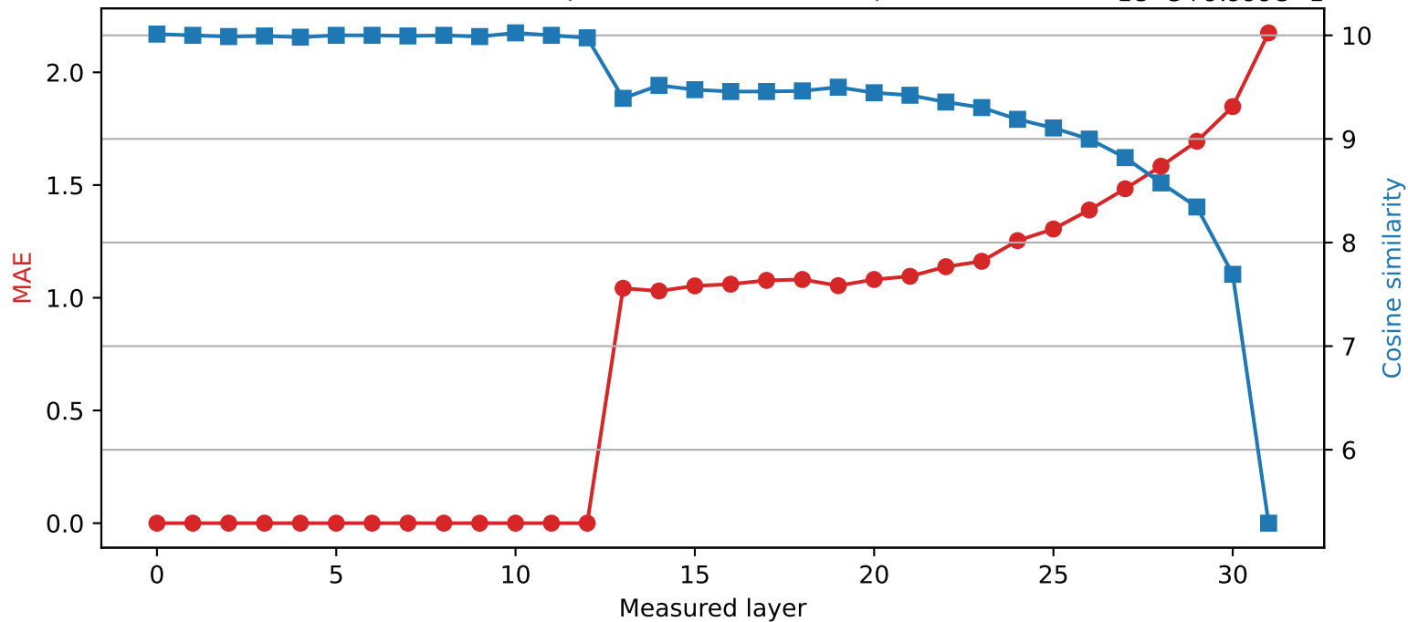
SmolLM2-360M | Quantized layer 12 | float32 → int2 1e-5+9.999e-1
