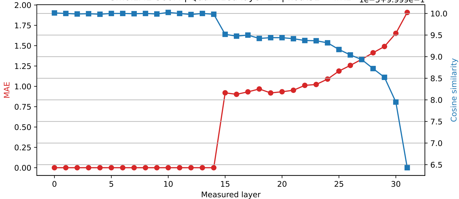
SmolLM2-360M | Quantized layer 14 | float32 \rightarrow int2 1e-5+9.999e-1
